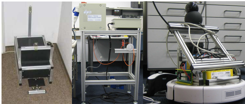
Fig. 4. Docking stations for the automatic battery charging. Left: VolksBot, Middle: Handycart. The arm is moving out if the robot it detected via infrared light, Right: The Roomba has an additional battery pack for the laser scanner and a digital relay card to switch power to the notebook if necessary.
